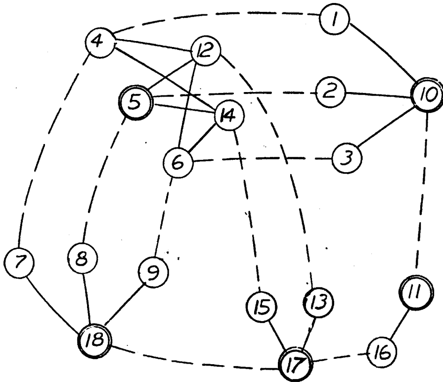
Figure VII.2: The layout graph for the routing shown in Figure 1. Conflict edges are solid (—), continuation edges are broken (---). Representative nodes are doubly circled for future reference.
