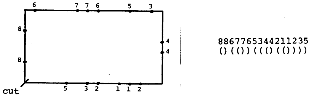
Figure IV.9: The correspondence between planar routing in a polygon (a) and parentheses expressions (b).
