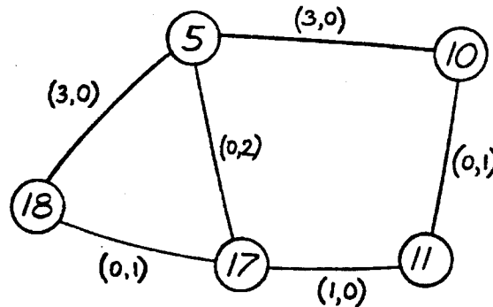
Figure VII.4: The residue graph corresponding to the layout of Figure 1, using the representatives as numbered in the nodes. A denotation (s, d) on an edge e means \sigma(e) = s , \delta(e) = d .
