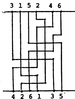
Figure V.16: Resolution of a non-tight set of nets involving three cycles.
