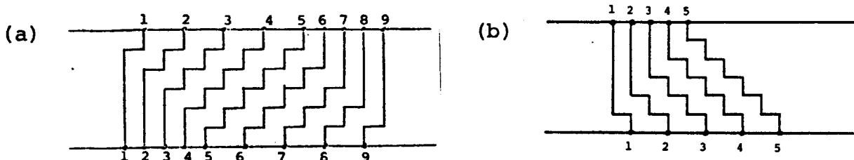
Figure V.8: River-routing: (a) shows a situation requiring \Omega(n^2) jogs, whereas in (b) more jogs than necessary are generated by the greedy algorithm.
