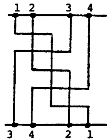
Figure V.14: Resolution of a single vertical conflict cycle.
