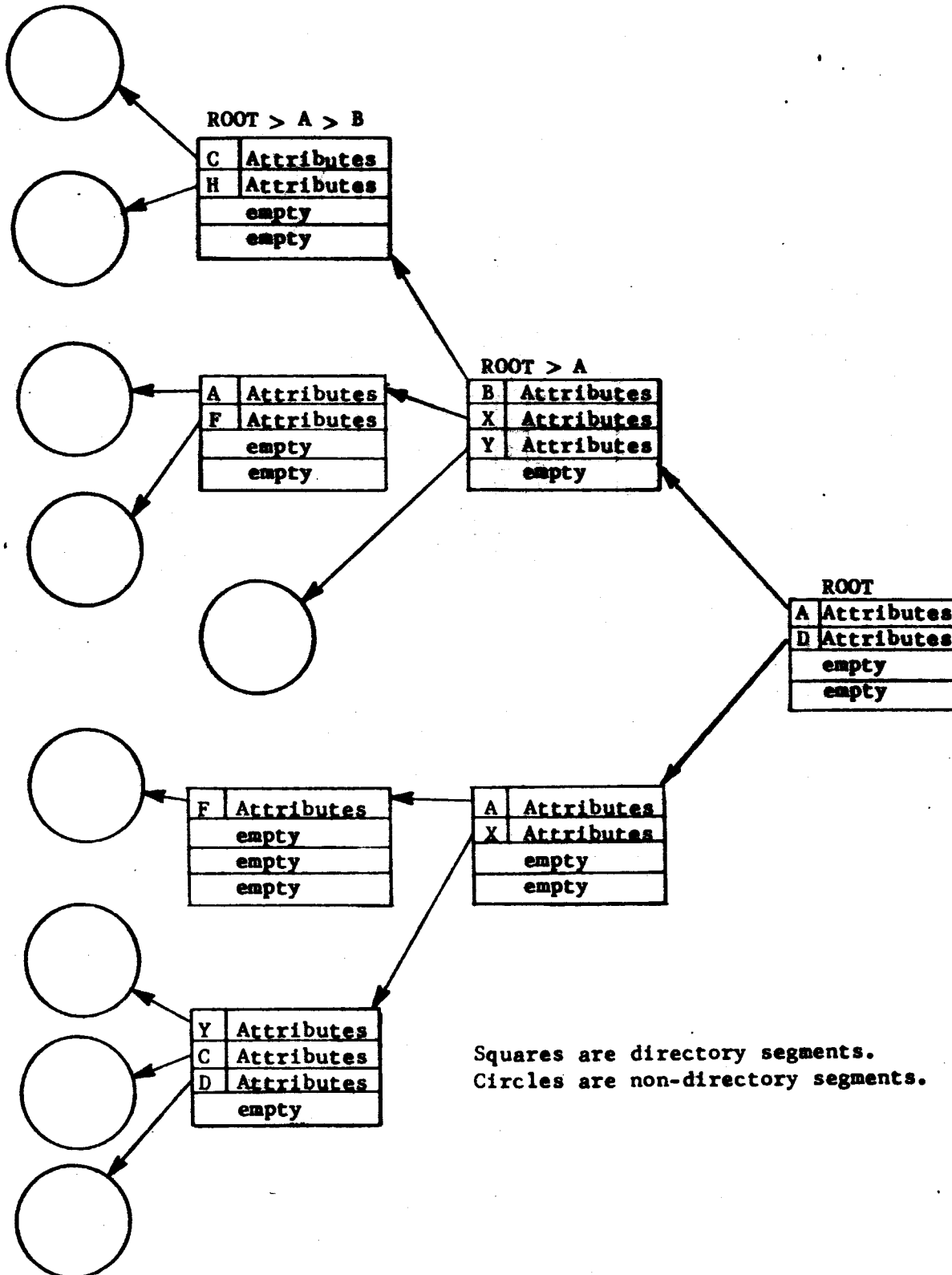
Figure 4. Directory Hierarchy
