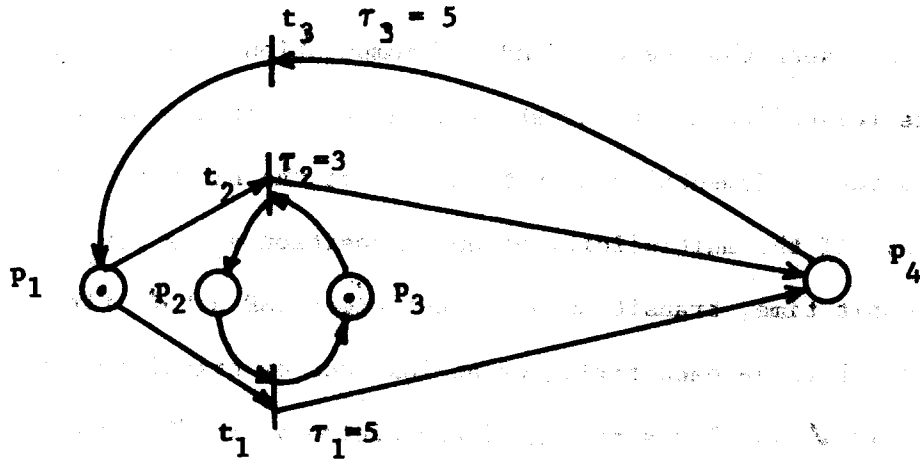
Figure 4.4.1 Timed LSP Petri net \mathcal{L} = \langle \mathcal{P}, \Omega \rangle with a live, bounded marking M .
