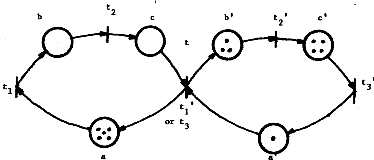
After firing t
