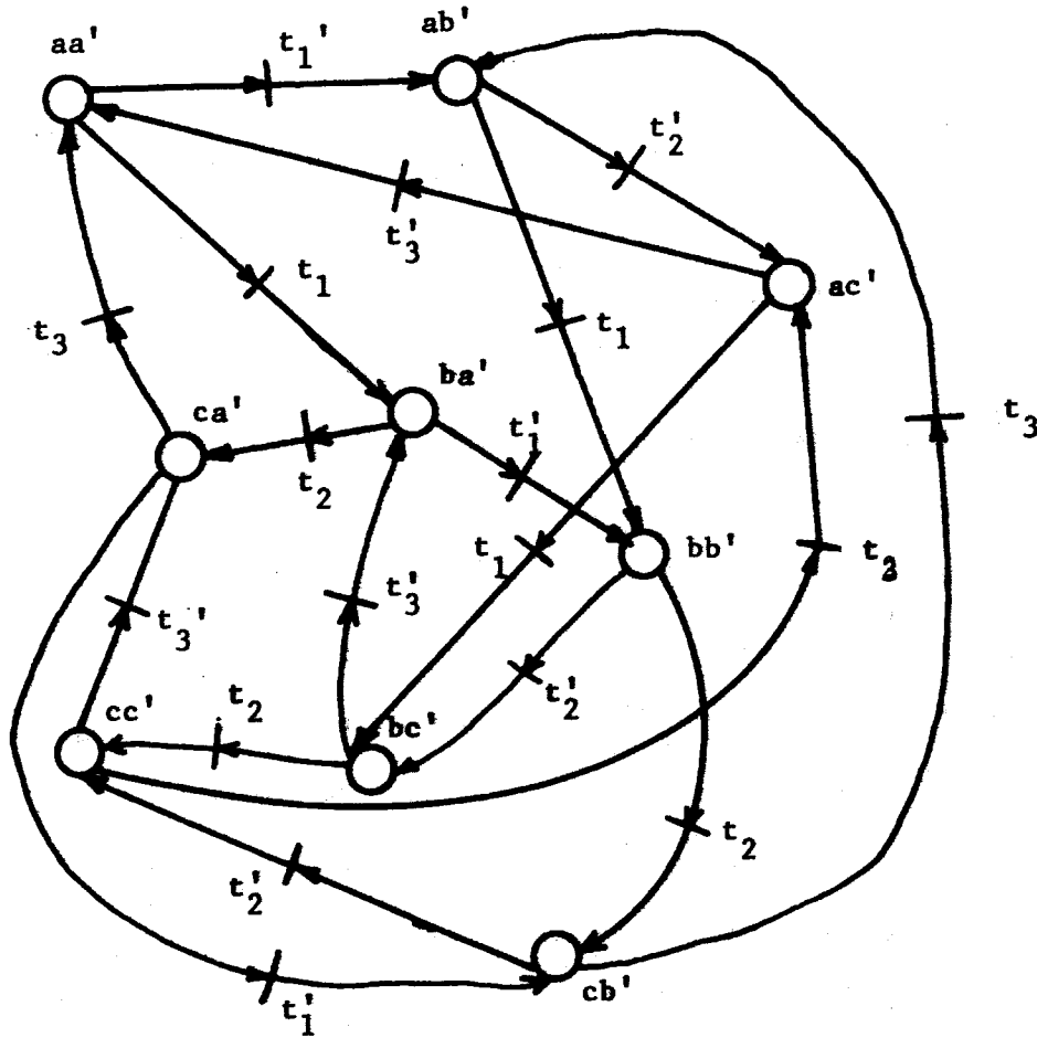
Figure 2.1.3 Finite State Machine Model of Pipelined Adder
