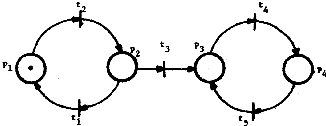
Figure 2.1.8 A finite state machine that is not strongly-connected.
