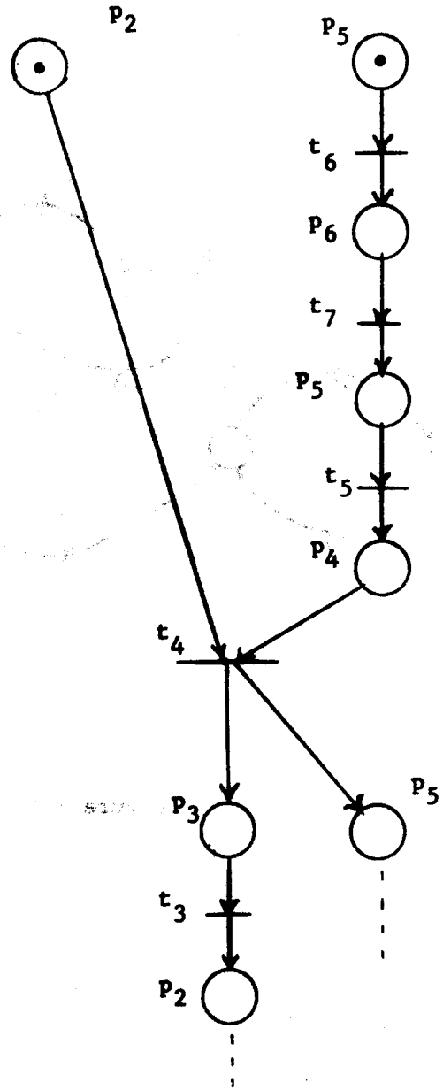
Occurrence Graph No. 2
