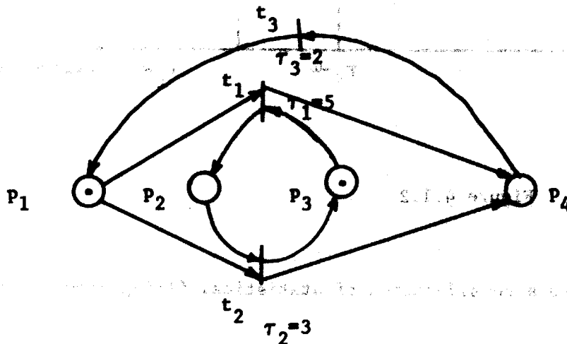
Figure 4.2.1 A Timed Petri net
