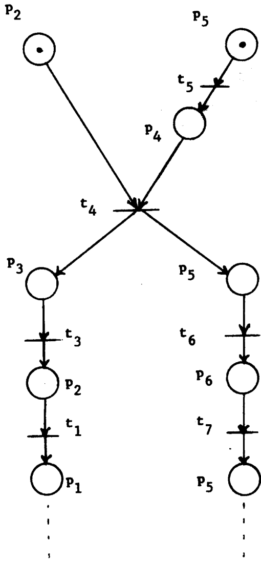
Occurrence Graph No. 1
