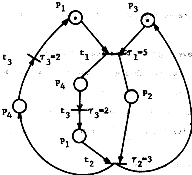
Figure 4.4.2 Steady state Equivalent net \mathcal{L} for LSP Petri net \mathcal{P} with marking M .
