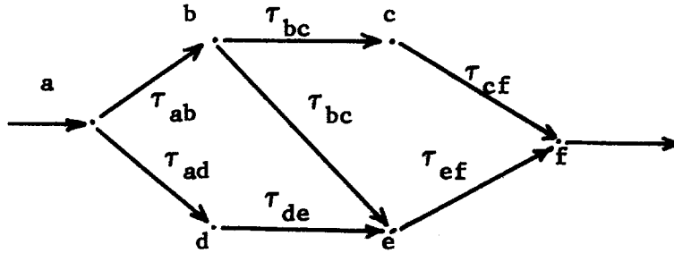
(a) A PERT Network.
