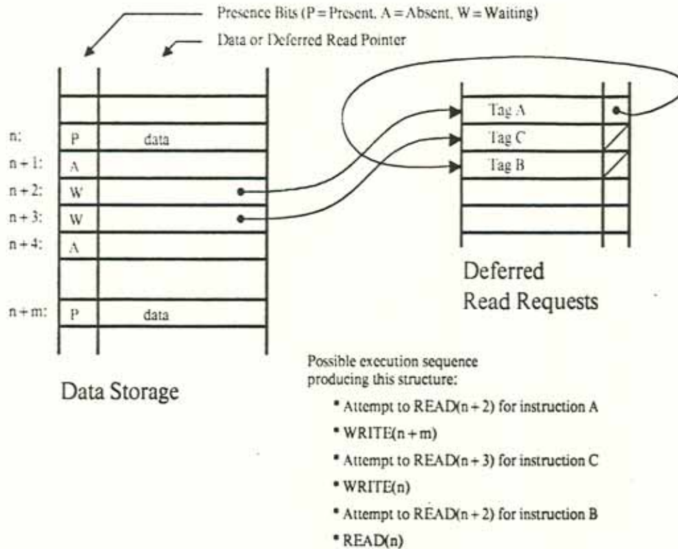
Figure 3-4: I-Structure Storage
