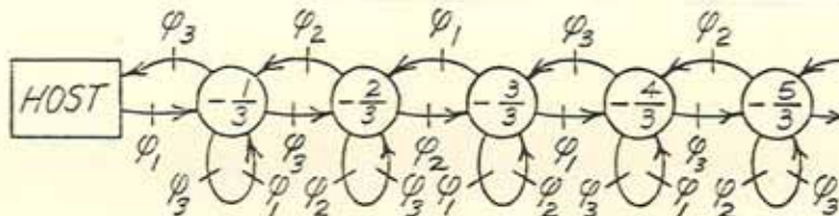
Figure 16: A fast implementation of the palindrome recognizer using three-phase clocking. Each vertex is labeled with its lag in this system with respect to P .
