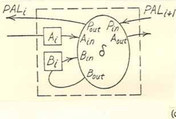
Figure 7: A synchronous system P which recognizes palindromes in real time. (a) A diagram of P showing registers and functional elements. The part enclosed in the dashed box corresponds roughly to a "processor" in the description of P in the text. (b) P 's communication graph, G . (c) Details of a functional element.
