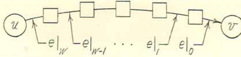
Figure 17: Division of an edge e = (u, v, w) into wires.
