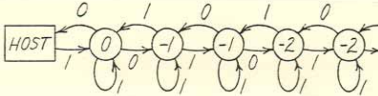
Figure 15: Communication graph of an optimized simulator for the real-time palindrome recognizer P of Figure 7. In the optimized simulator, no signal propagates through more than two functional elements in one clock period. Each vertex is labeled with its lag in this system with respect to P .
