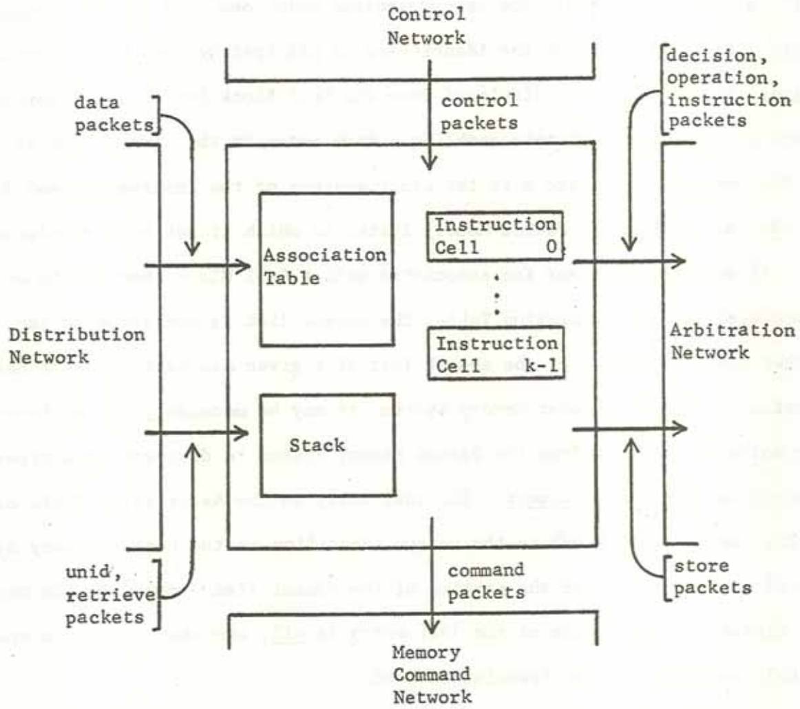
Figure 3.15. Organization of an Instruction Cell Block.
