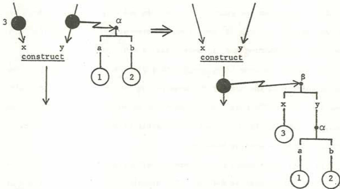
Figure 2.5. Operation of the construct actor.
