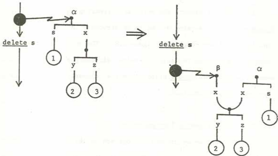
Figure 2.8. Operation of the delete actor.
