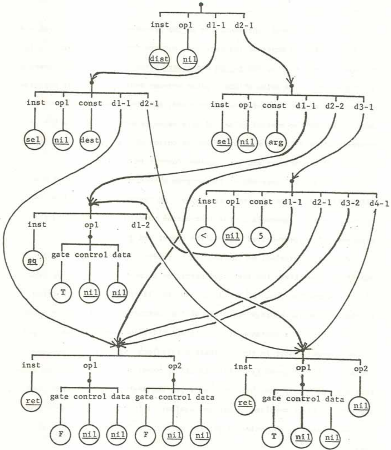
Figure 2.11. Structured representation of the program of Figure 2.10.
