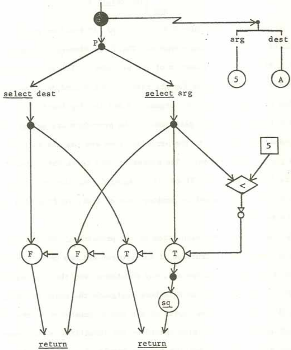
Figure 2.10. Data-flow representation of a simple procedure.
